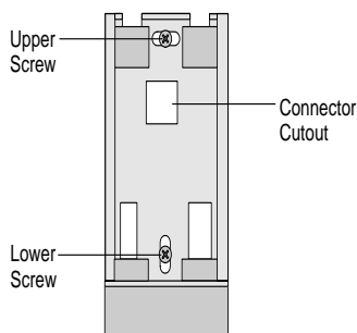
Figure 16 Bracket Mounted onto the Wall
